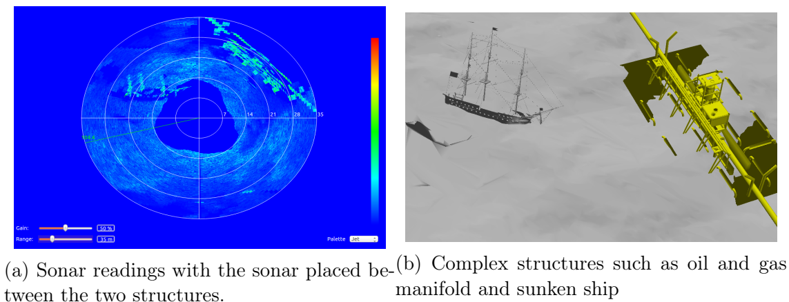
Figure 4.6: Sonar Simulation in a unstructured environment.
