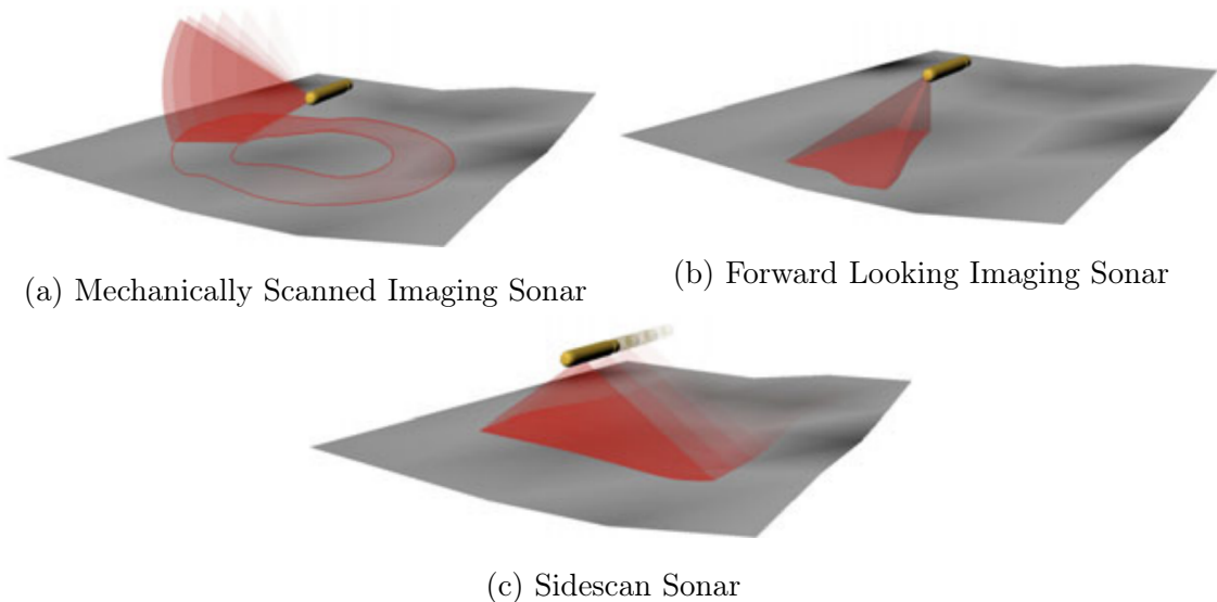
Figure 2.14: Most common active sonar types (adapted from [52]).
