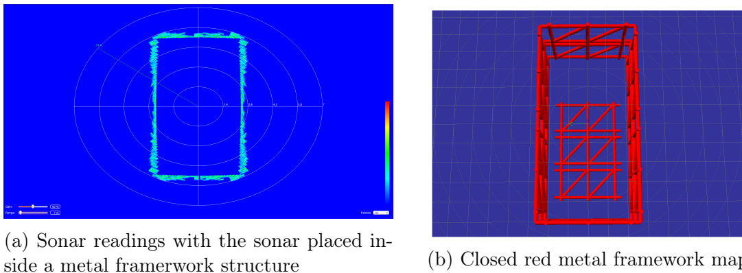
Figure 4.5: Sonar Simulation in an structured environment.
