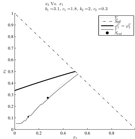
Figure D.2: Trajectory on the phase plane showing more than one crossing. This situation does not comply with Filippov’s theory for Odes with discontinuous RHS.
