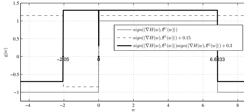
Figure 5.9: Model LVsP, scenario 3: Signs of the inner products used in the calculation of conditions for crossing and sliding.
