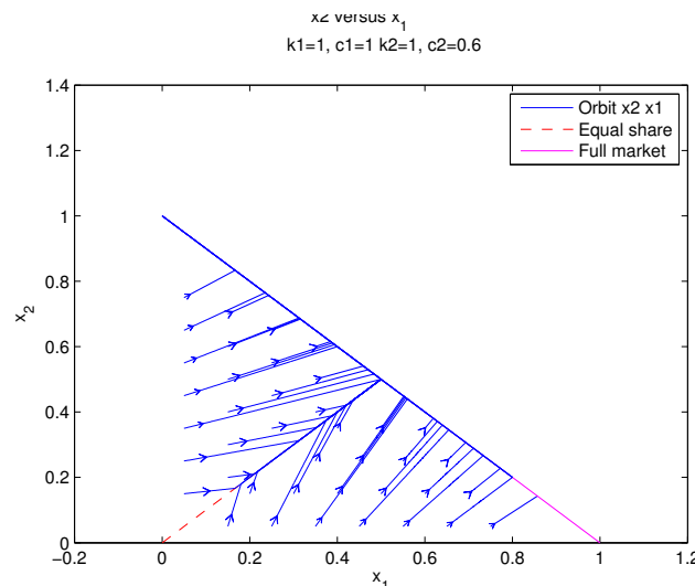
Figure D.1: Simulation ran with Piironen, Kuznetsov Matlab software. Trajectories should stop on the saturated line Sat , however in the simulation they continue moving upwards.
