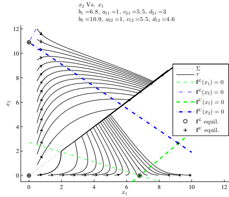
Figure 5.11: Model LVsP, scenario 4: Same simulation as in Figure 5.10, but here the stepsiz = 0.0002 is smaller and this reduces most of the chattering on the equal number of clients line \Sigma .
