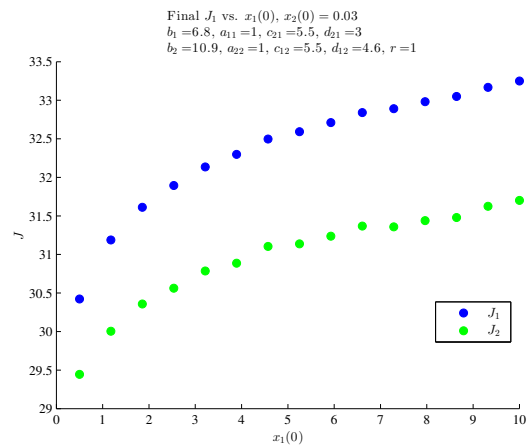
Figure 5.22: Model LVsP, scenario 4: Value of indices when the initial value x_2(0) = 0.03 is fixed.
