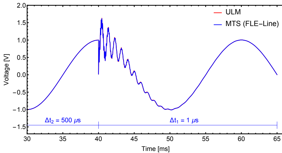
Figure 2.31: Case #4: Simulated voltage at terminal # 4
