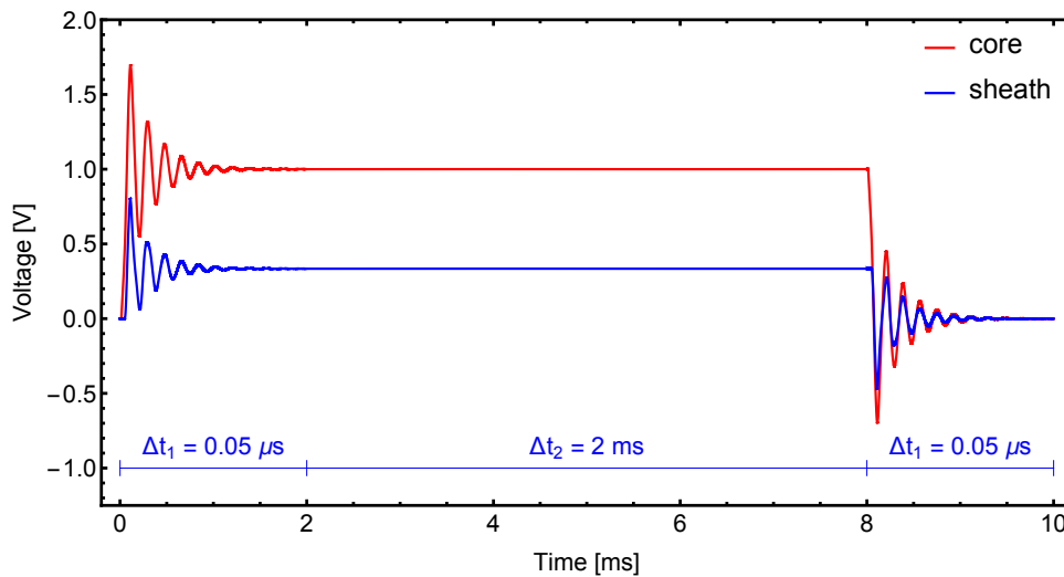
Figure 3.37: Case #6: Simulated core and sheath voltages
