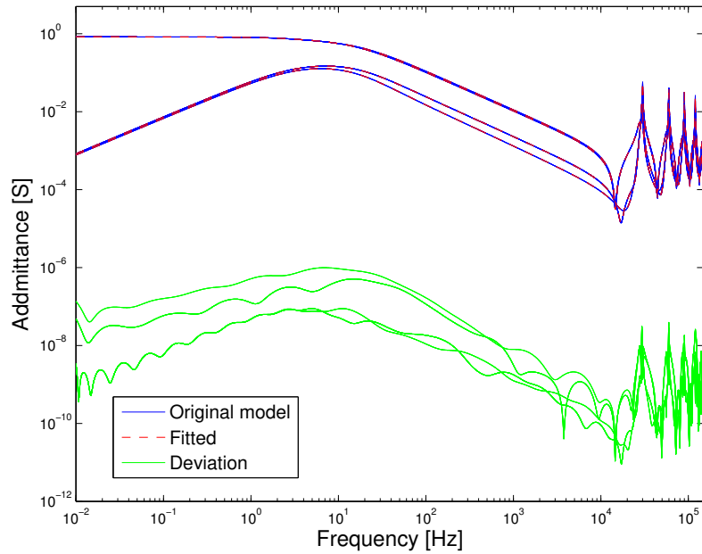
(a) Fitting of M_1
