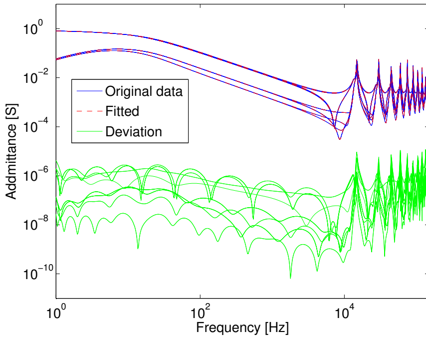
(a) Fitting of \mathbf{Y}_n
