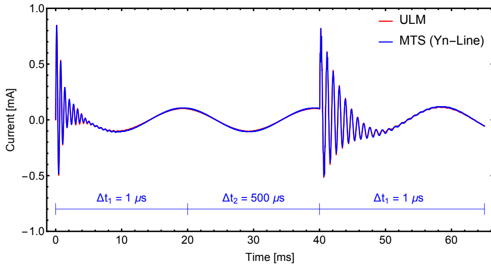
(a) Current at terminal # 1
