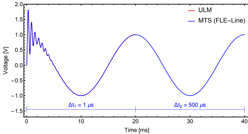
Figure 2.30: Case #4: Simulated voltage at terminal # 4
