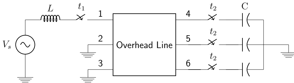
Figure 3.28: Case #5: Circuit for time-domain simulation
