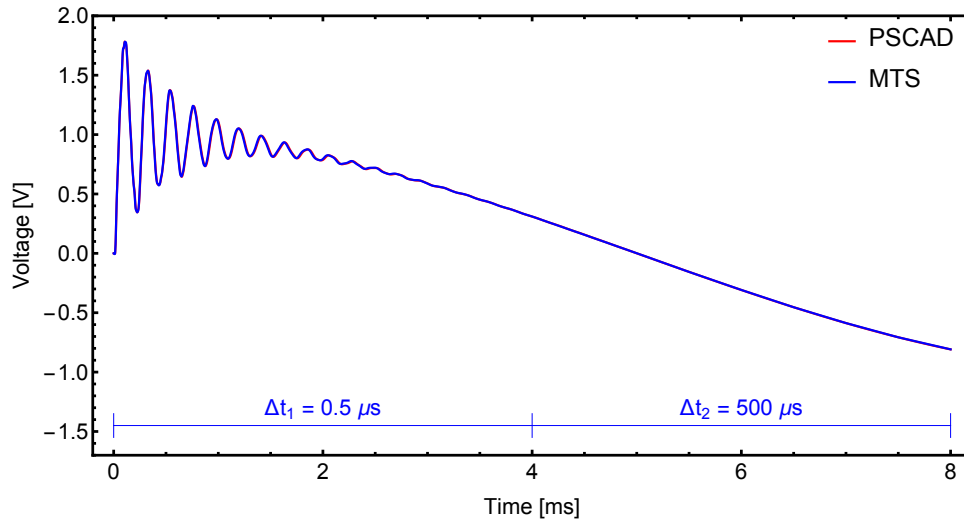
Figure 2.15: Case #2: Simulated voltage at terminal # 4
