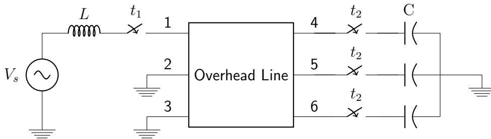
Figure 3.16: Case #3: Circuit for time-domain simulation
