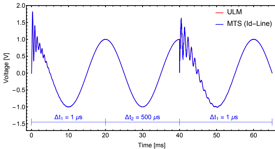
Figure 2.38: Case #5: Simulated voltage at terminal # 4
