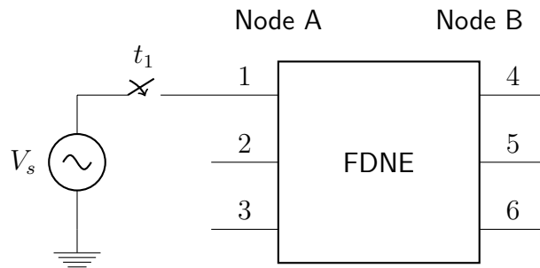
Figure 2.14: Case #2: Circuit for time-domain simulation
