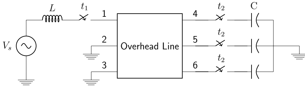
Figure 2.35: Case #5: Circuit for time-domain simulation
