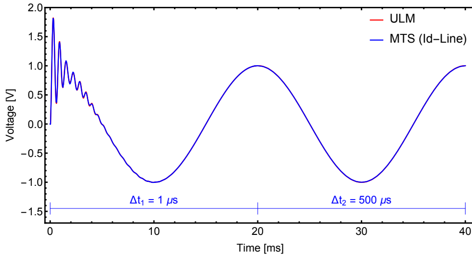
Figure 2.36: Case #5: Simulated voltage at terminal # 4
