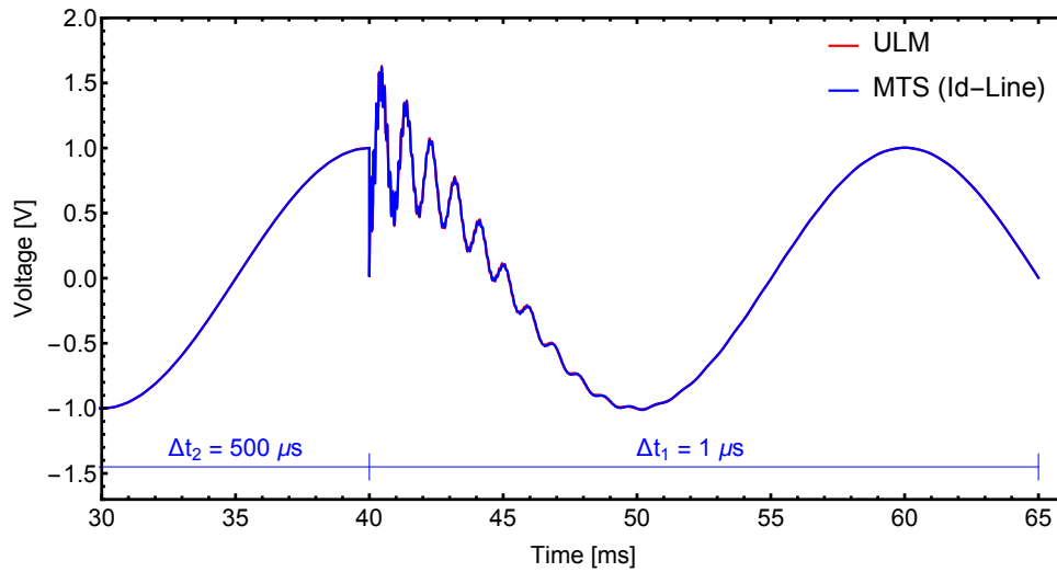
Figure 2.37: Case #5: Simulated voltage at terminal # 4
