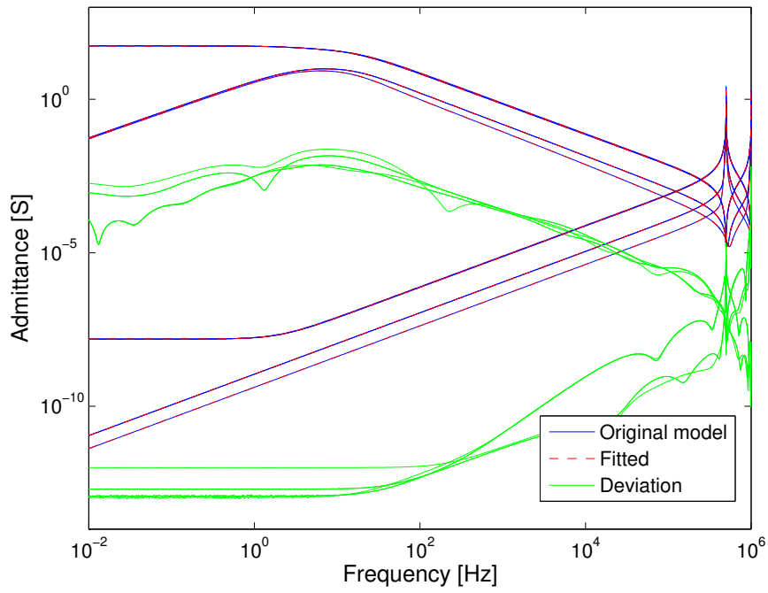
(a) Fitting of \mathbf{Y}_{oc} and \mathbf{Y}_{sc}
