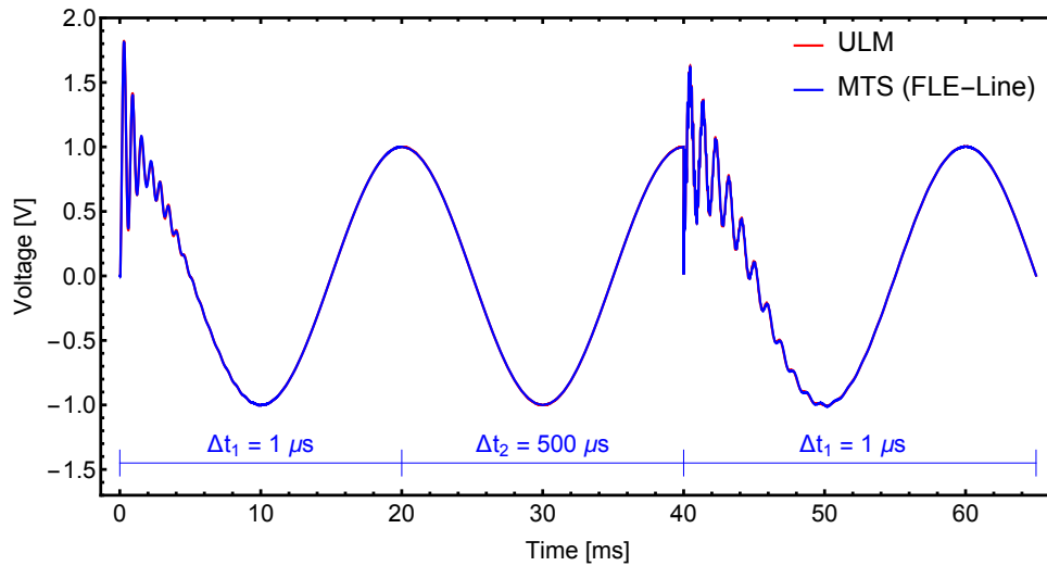
Figure 2.32: Case #4: Simulated voltage at terminal # 4
