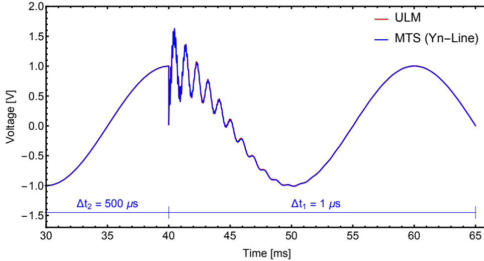
Figure 2.24: Case #3: Simulated voltage at terminal # 4
