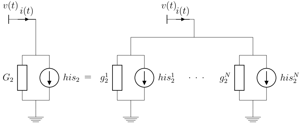
Figure 2.6: Sketch for time step transition
